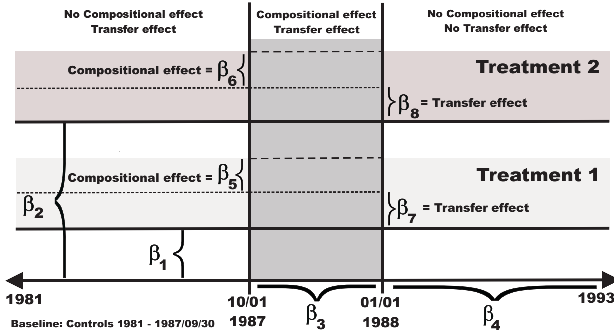
Figure 5: Research design
