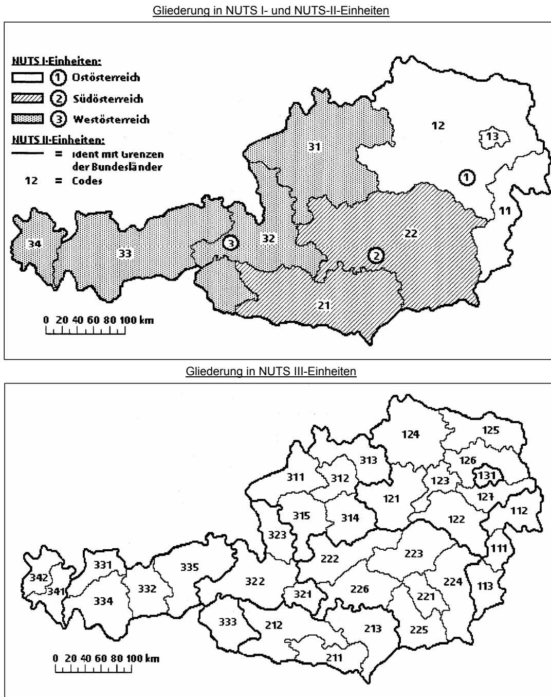
Figure 1: Geographical representation of the nuts -classification
